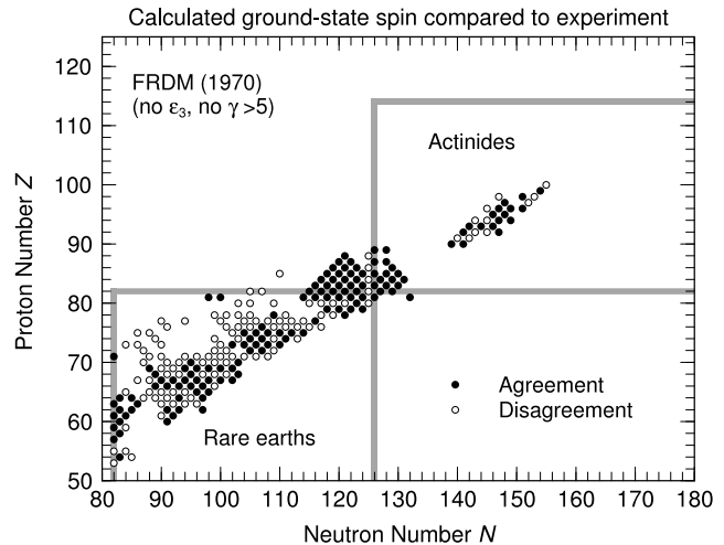
Fig. 2. Calculated spins for o–e nuclides compared to experiment in the heavy-mass regions. The calculations are carried out with the original 1970 spin–orbit and diffuseness parameter values, see text. Magic proton and neutron numbers are indicated by wide, gray lines.
