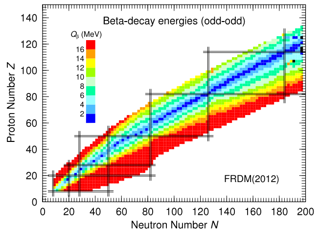
Fig. 12. Calculated \beta -decay energies Q_\beta for o–o parents. To avoid squares with no color, each e–e nucleus at Z and N is represented by a square with corners in (N + 1, Z - 1) , (N + 1, Z + 1) , (N - 1, Z + 1) and (N - 1, Z - 1) , just as was the case with the e–e parent plot. Since there are no \beta -stable o–o nuclei there are no black squares in this figure. Magic proton and neutron numbers are indicated by wide, gray lines. (For a colour version of this figure the reader is referred to the web version of this article.)
