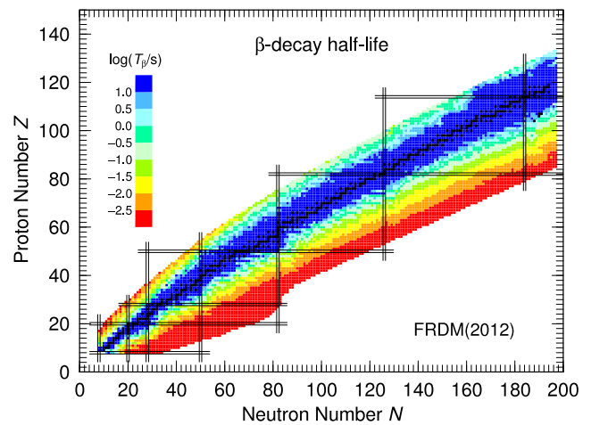
Fig. 22. Calculated \beta -decay half-lives. Magic proton and neutron numbers are indicated by wide, gray lines.
