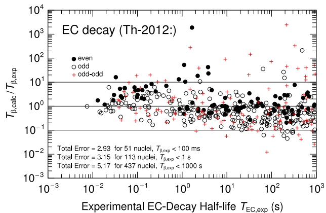
Fig. 21. Ratio between calculated and measured electron-capture half-lives plotted versus experimental electron-capture half-life.
