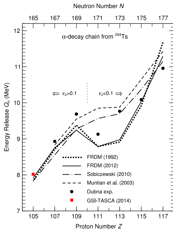
Fig. 30. Calculated and measured Q_{\alpha} -decay energies in the decay chain originating in ^{294}\text{Ts} . The calculated values assume ground-state to ground-state decay, the measured energies may not be, so the differences between measured and calculated values do not directly indicate the degree of (in)accuracy of the underlying mass model. Note that in one of the models the kink observed in the experimental data at Z = 109 – 111 is well reproduced. In this case the kink is related to a change in deformation from spherical to deformed, rather than a gap in the level spectrum at a fixed deformation. Source: The experimental data are from [49,70]. The calculated data are from [71–73].
