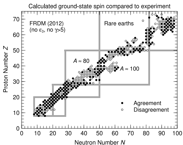
Fig. 3. Calculated spins for o–e nuclides compared to experiment in the light- and medium-mass regions. The calculations are carried out with the current (same since 1974/1981) spin–orbit and diffuseness parameter values, see text. Magic proton and neutron numbers are indicated by wide, gray lines.
