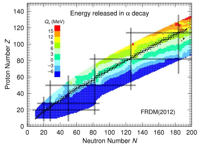
Fig. 27. Energy Q_{\alpha} released in \alpha -decay for ground-state to ground-state transitions. Black squares are \beta -stable nuclei. Magic proton and neutron numbers are indicated by pairs of parallel lines. (For a colour version of this figure the reader is referred to the web version of this article.)
