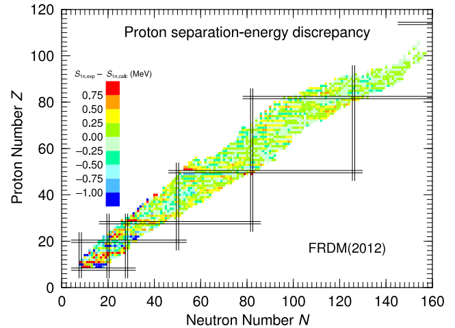
Fig. 26. Discrepancy between experimental and calculated one-proton separation-energies. Magic proton and neutron numbers are indicated by pairs of parallel lines. Large discrepancies occur where there are large changes in the deviations between calculated and experimental masses between neighboring nuclei, namely at some magic numbers and in the region of light nuclei. In the deformed rare-earth and actinide regions the discrepancy is very small. (For a colour version of this figure the reader is referred to the web version of this article.)
