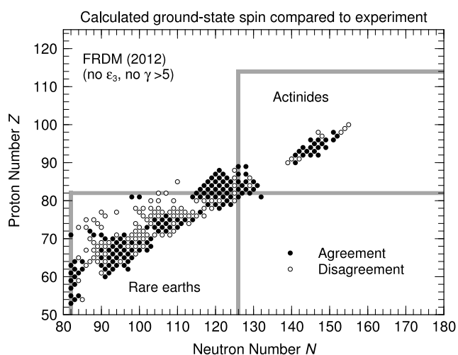
Fig. 4. Calculated spins for o–e nuclides compared to experiment in the heavy-mass regions. The calculations are carried out with the current (same since 1974/1981) spin–orbit and diffuseness parameter values, see text. Magic proton and neutron numbers are indicated by wide, gray lines.
