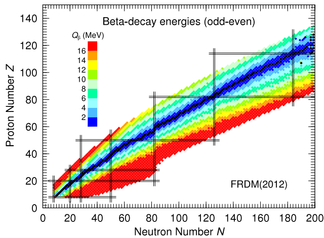
Fig. 10. Calculated \beta -decay energies Q_\beta for o–e parents. To avoid squares with no color, each o–e nucleus at Z and N is represented by a square with corners in (N + 1, Z) , (N + 1, Z + 1) , (N - 1, Z) and (N - 1, Z + 1) . The o–e \beta -stable nuclei are similarly represented. Magic proton and neutron numbers are indicated by wide, gray lines. (For a colour version of this figure the reader is referred to the web version of this article.)
