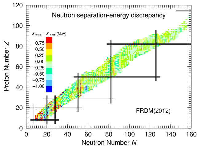
Fig. 8. Discrepancy between experimental and calculated one-neutron separation energies. Magic proton and neutron numbers are indicated by pairs of parallel lines. Large discrepancies occur where there are large changes in the deviations between calculated and experimental masses between neighboring nuclei, namely at some magic numbers and in the light region of nuclei. In the deformed rare-earth and actinide regions the discrepancy is very small. (For a colour version of this figure the reader is referred to the web version of this article.)
