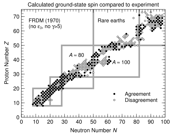
Fig. 1. Calculated spins for o–e nuclides compared to experiment in the light- and medium-mass regions. The calculations are carried out with the original 1970 spin–orbit and diffuseness parameter values, see text. Magic proton and neutron numbers are indicated by wide, gray lines.
