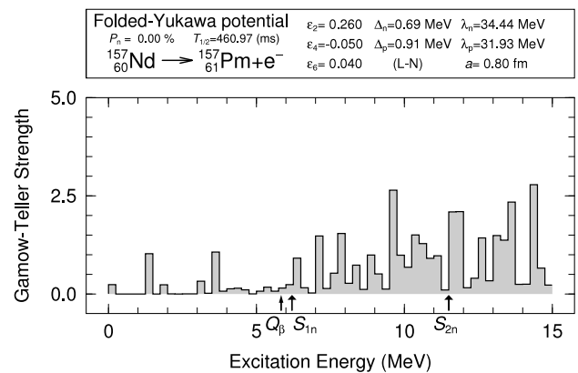
Fig. 14. Calculated Gamow–Teller \beta -strength function for ^{157}\text{Nd} .
