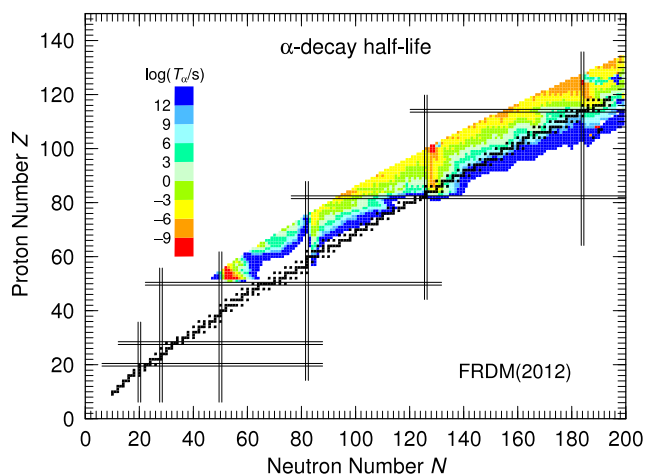
Fig. 28. Half-life with respect to \alpha -decay calculated from a semiempirical relationship between T_{\alpha} and Q_{\alpha} . Black squares are \beta -stable nuclei. Magic proton and neutron numbers are indicated by pairs of parallel lines. (For a colour version of this figure the reader is referred to the web version of this article.)
