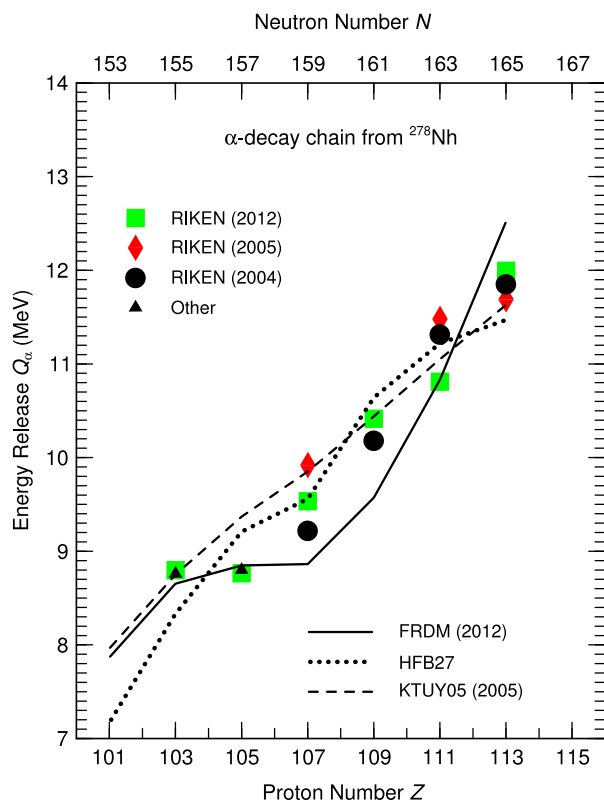
Fig. 29. Calculated and measured Q_{\alpha} -decay energies in the decay chain originating in ^{278}\text{Nh} . The calculated values assume ground-state to ground-state decay, the measured energies may not be, so the differences between measured and calculated values do not directly indicate the degree of (in)accuracy of the underlying mass model. Note that in one of the models the kink observed in the experimental data at Z \approx 108 is well reproduced. Source: The measured data are from [45–47]. The KTUY05 calculation is from [68,69].
