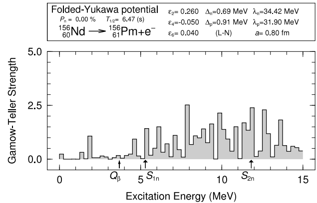
Fig. 13. Calculated Gamow–Teller \beta -strength function for ^{156}\text{Nd} . The narrow arrow indicates the Q_\beta energy, the wide arrows the neutron separation energies S_{1n} and S_{2n} .
