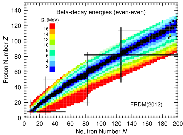
Fig. 11. Calculated \beta -decay energies Q_\beta for e–e parents. To avoid squares with no color, each e–e nucleus at Z and N is represented by a square with corners in (N + 1, Z - 1) , (N + 1, Z + 1) , (N - 1, Z + 1) and (N - 1, Z - 1) . The e–e \beta -stable nuclei are similarly represented. Magic proton and neutron numbers are indicated by wide, gray lines. (For a colour version of this figure the reader is referred to the web version of this article.)
