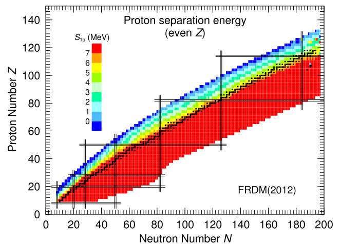
Fig. 24. Proton separation energy S_{1p} for even Z . Each color square is two protons high and one neutron wide. Magic proton and neutron numbers are indicated by wide, gray lines. (For a colour version of this figure the reader is referred to the web version of this article.)
