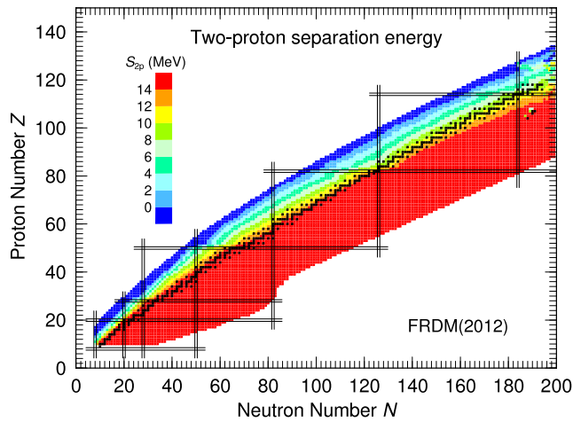
Fig. 25. Two-proton separation energy S_{2p} . Each color square is one proton high and one neutron wide. Magic proton and neutron numbers are indicated by wide, gray lines. (For a colour version of this figure the reader is referred to the web version of this article.)
